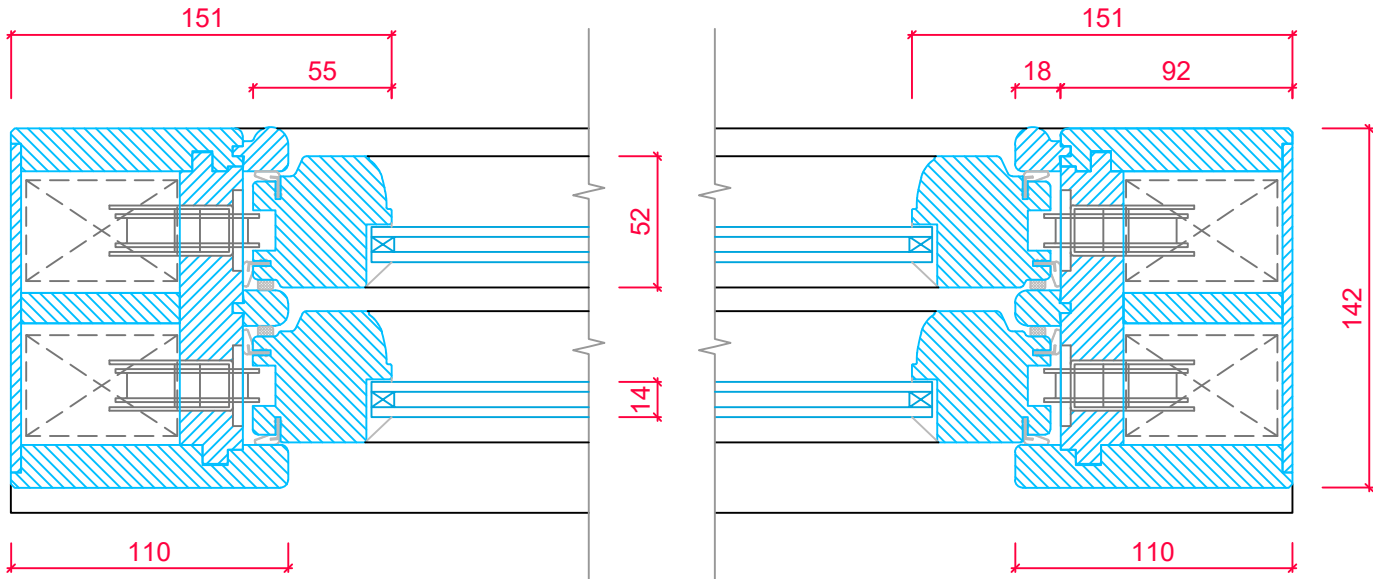
SASH CROSS SECTION 'A-A'
