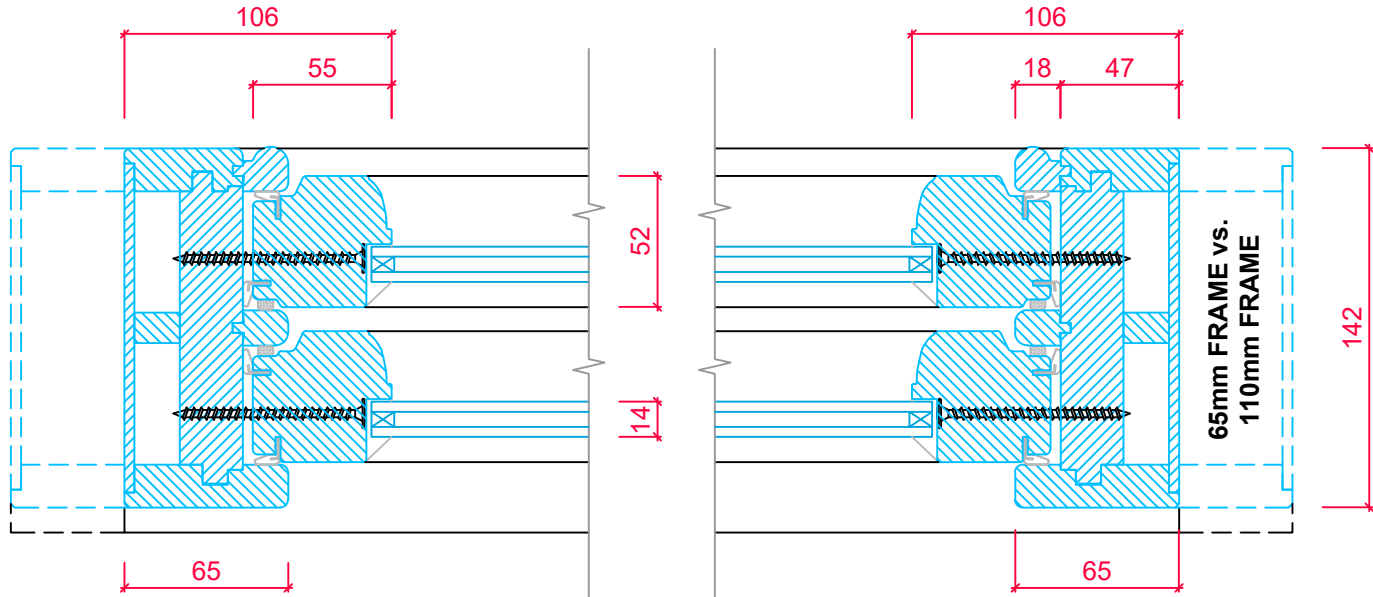
SASH CROSS SECTION 'B-B' 65mm FRAME ONLY AVAILABLE ON FIXED SASHES
