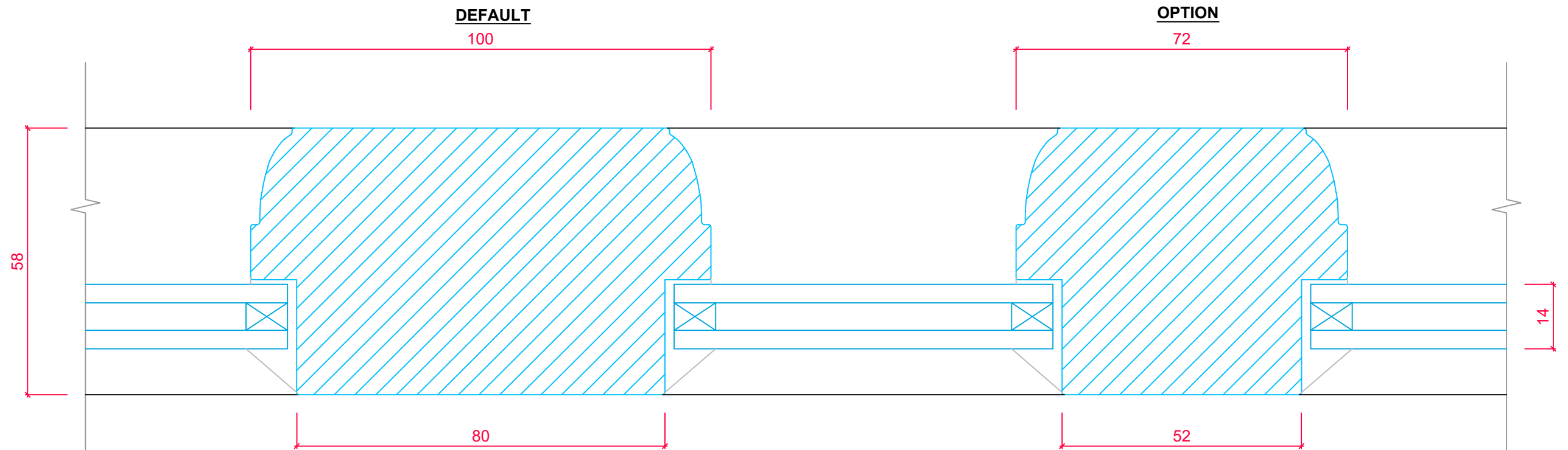
FRAME CROSS SECTION 'A-A'
