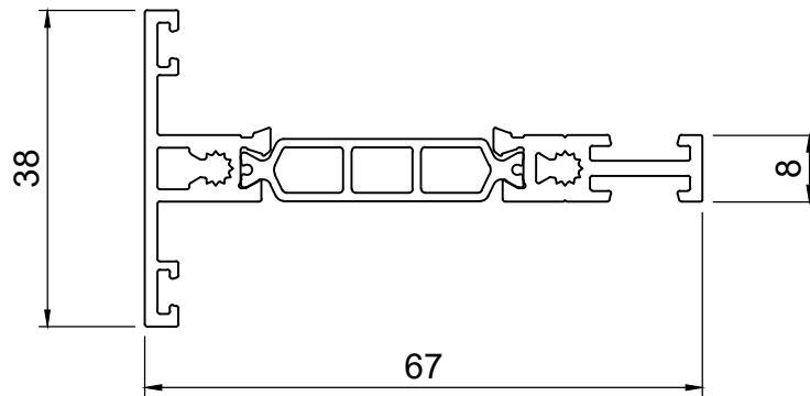
38mm Transom / Mullion
