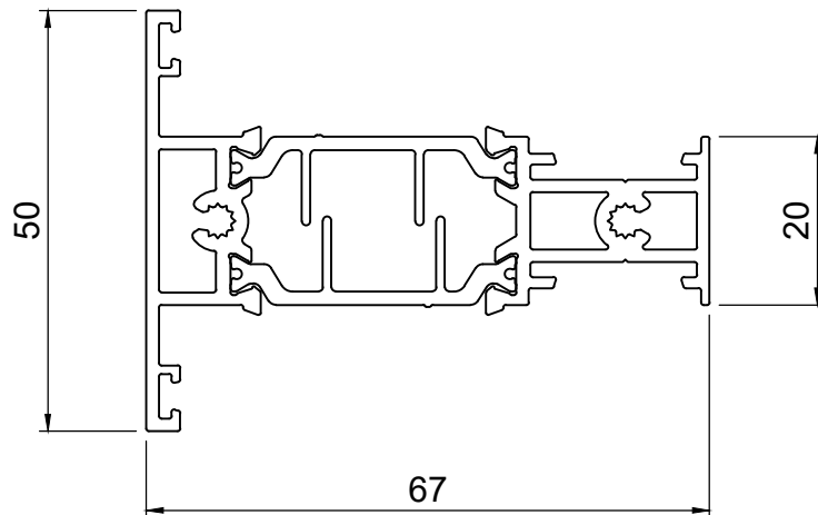
50mm Transom / Mullion
