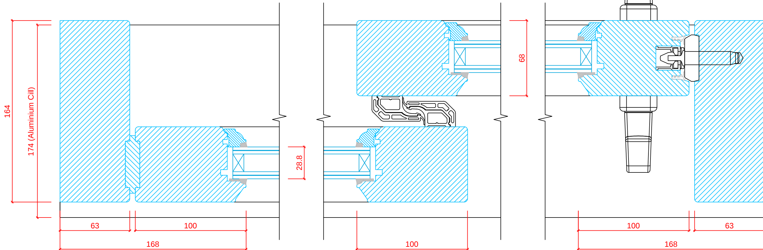
FRAME CROSS SECTION 'A-A'
