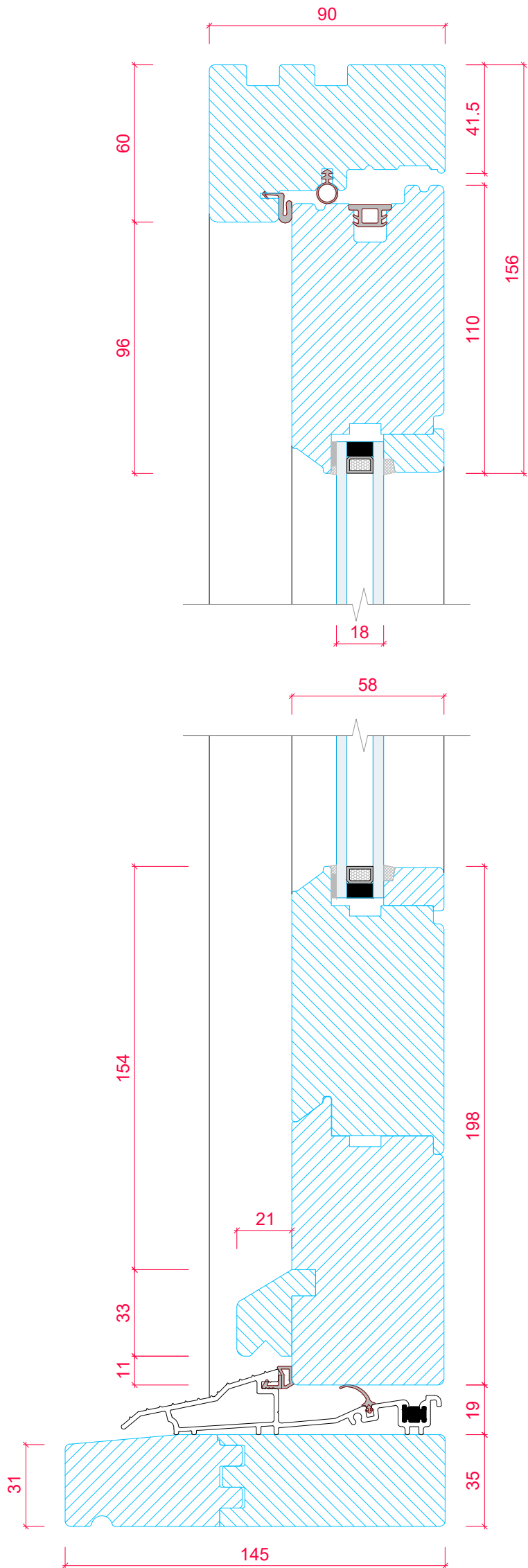
ENTRANCE DOOR CROSS SECTION 'A-A' (SCALE 1:2)
