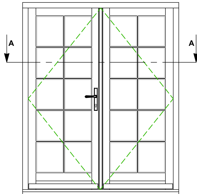
TYPICAL FRAME LAYOUT
