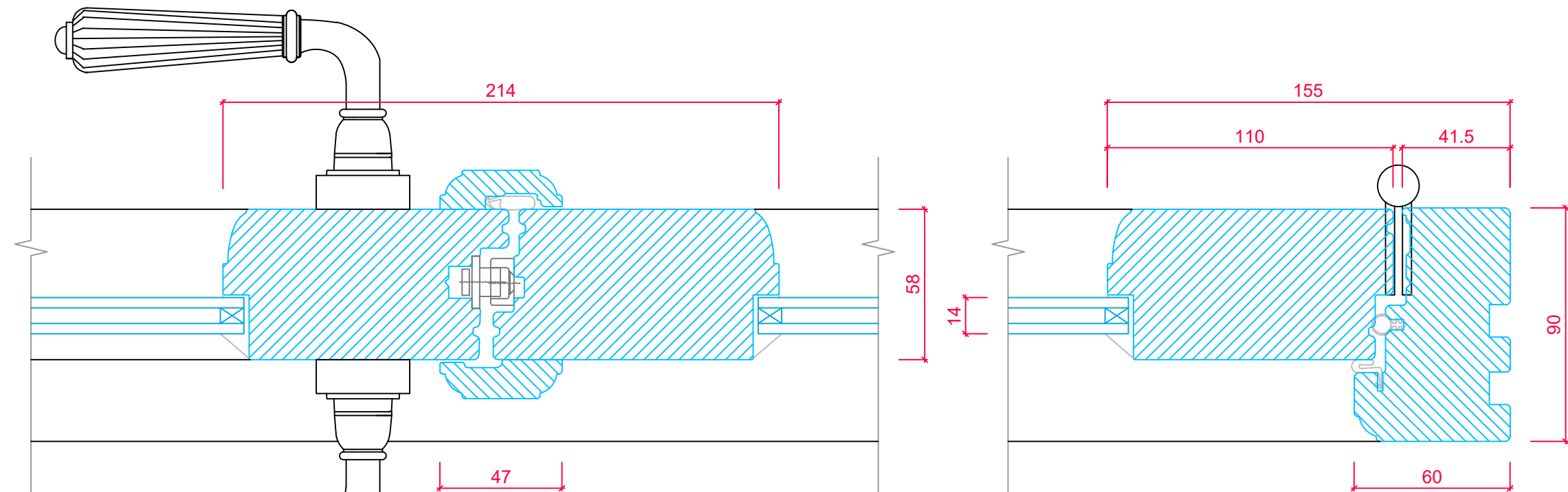
FRAME CROSS SECTION 'A-A'
