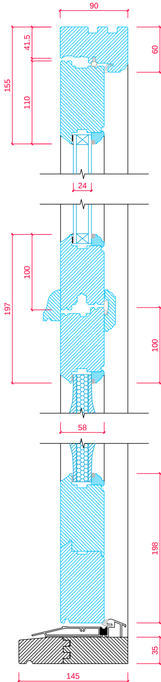
FRAME CROSS SECTION 'A-A'
