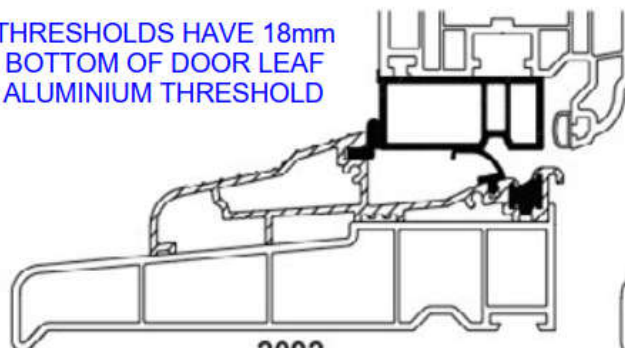
2092 AM3 SUB-CILL THRESHOLD OPEN IN END CAPS L2090
