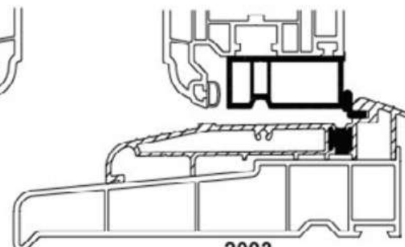
2093 AM5EX SUB CILL THRESHOLD OPEN OUT END CAPS L2097
