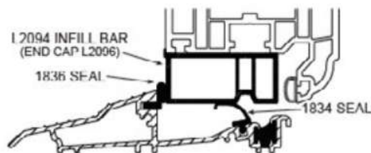
2090 AM3 THRESHOLD OPEN IN END CAPS L2098
