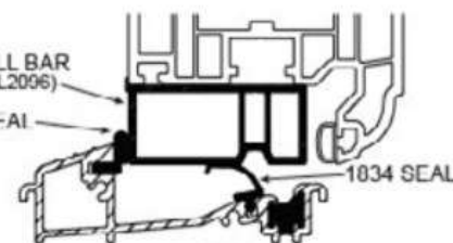
2099 AM3 70 THRESHOLD OPEN IN END CAPS L2101
