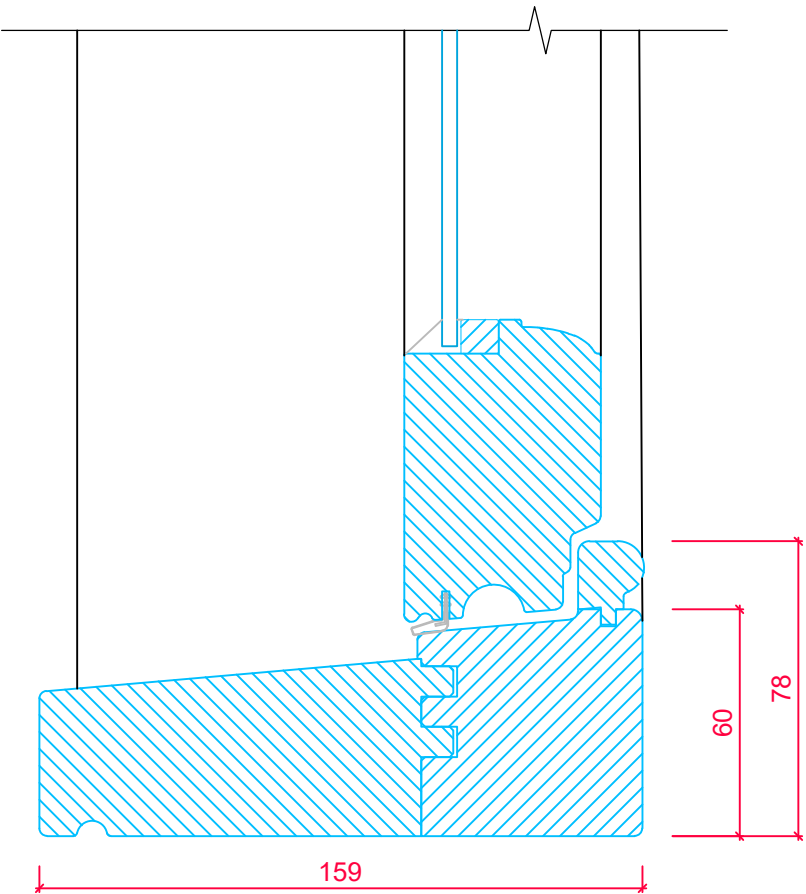
STANDARD CILL OPTION SECTION 'A-A'
