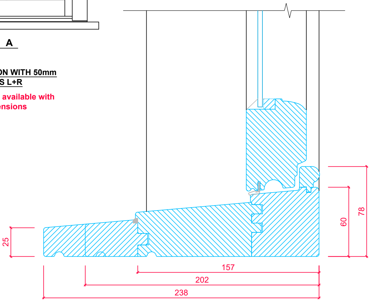
CILL EXTENSION OPTIONS SECTION 'A-A'
