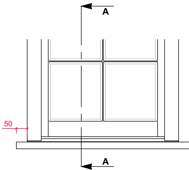
CILL ELEVATION WITH 50mm HORNS L+R
