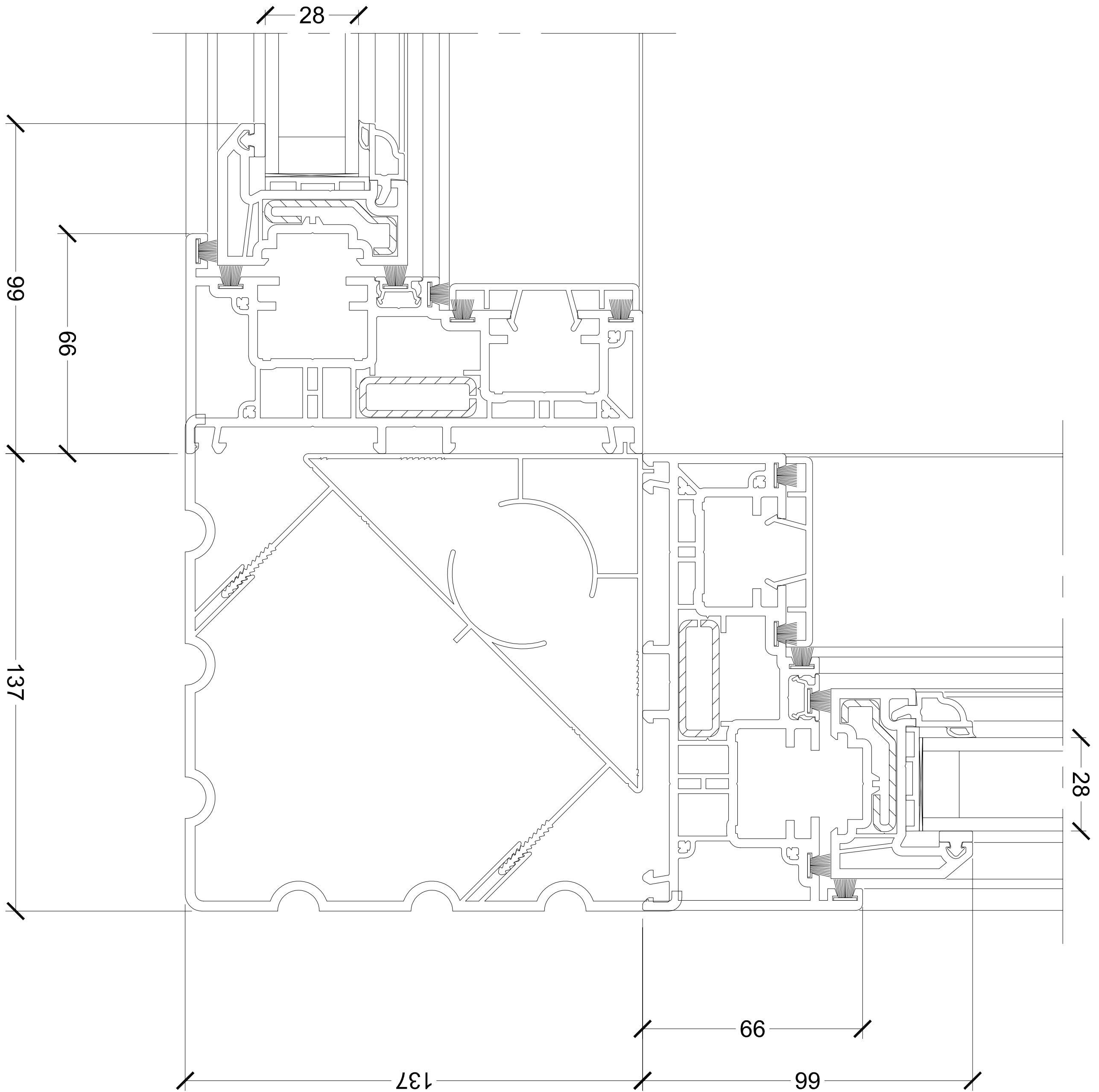
D-D Section Detail Scale 1:2
