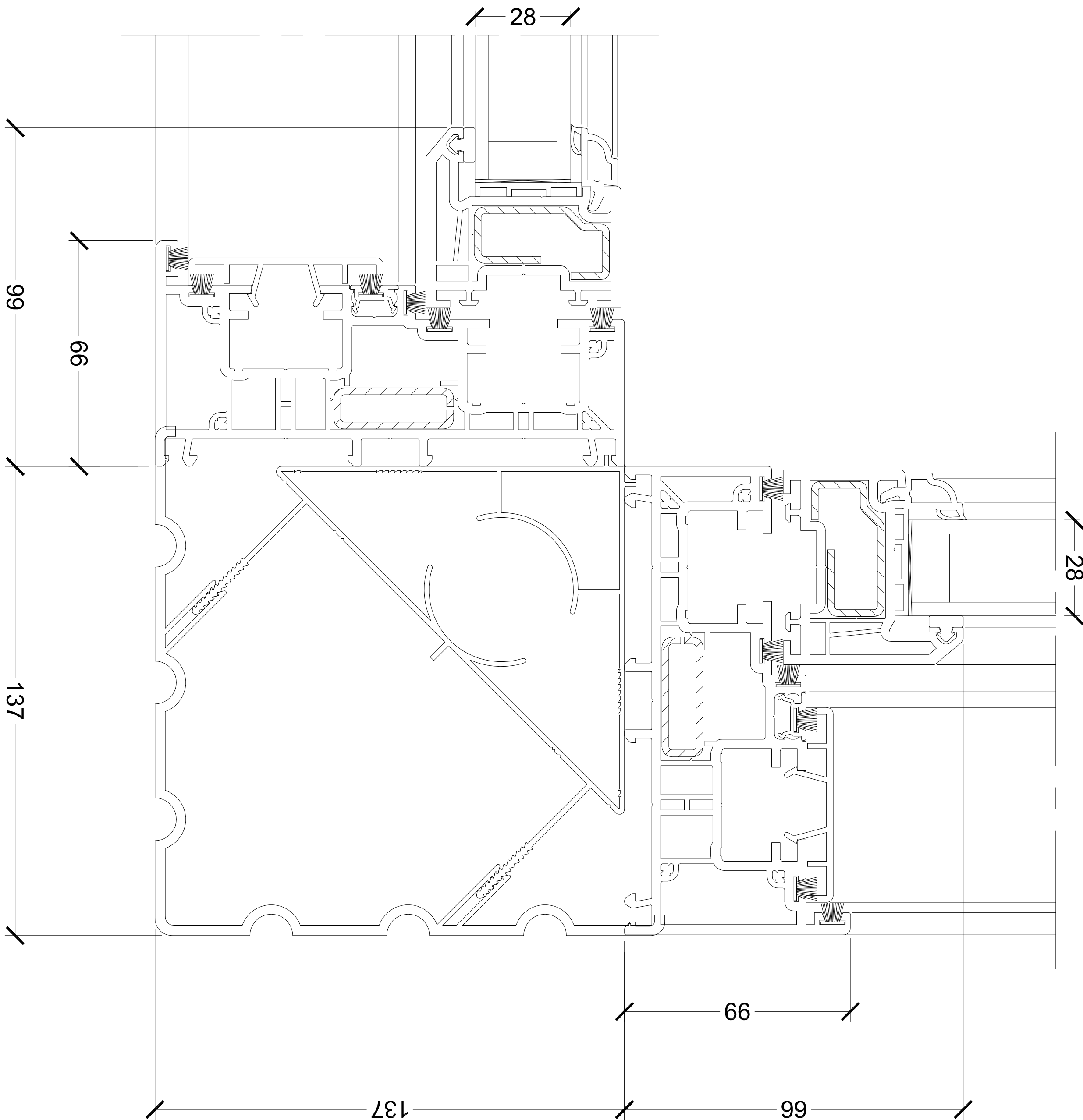
E-E Section Detail Scale 1:2
