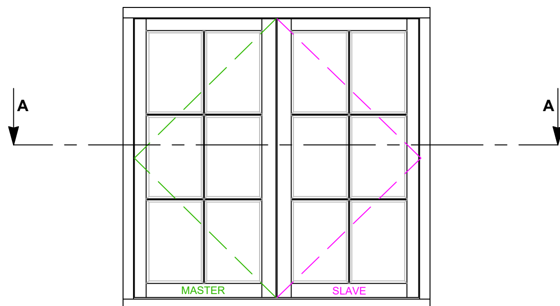
TYPICAL CASEMENT LAYOUT
