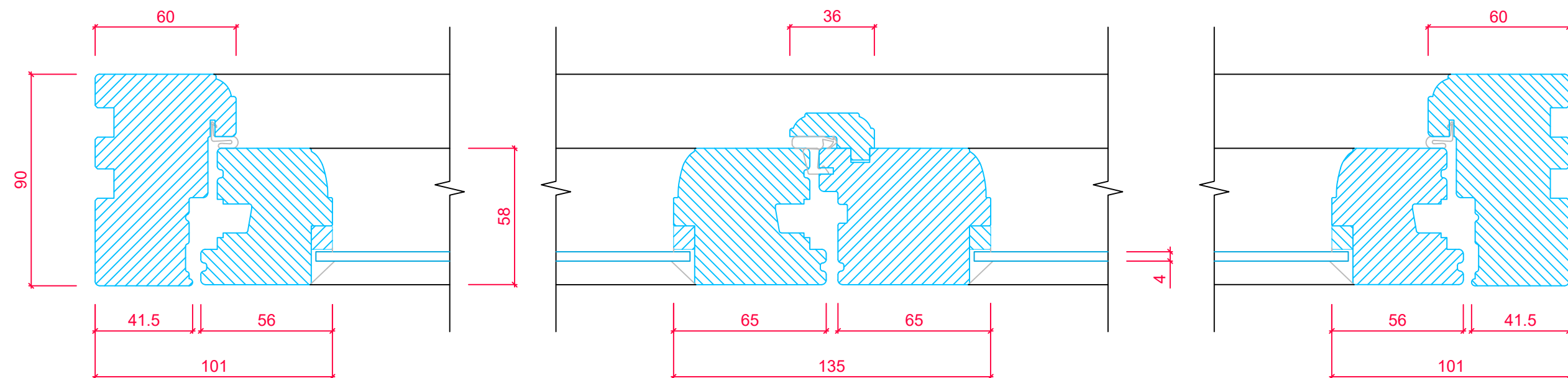
CASEMENT CROSS SECTION 'A-A'
