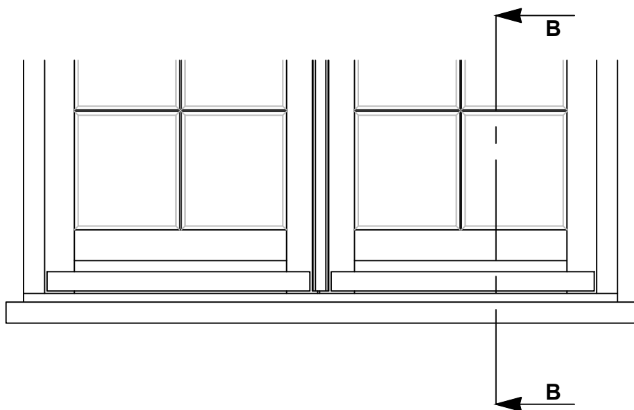
60mm CILL ELEVATION WITH 50mm HORNS L+R
