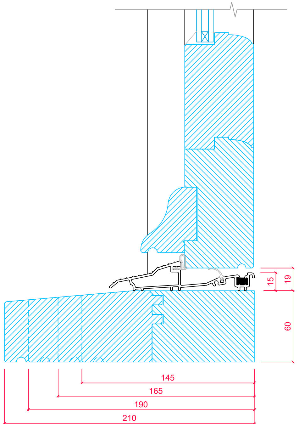
60mm CILL OPTIONS SECTION 'B-B'
