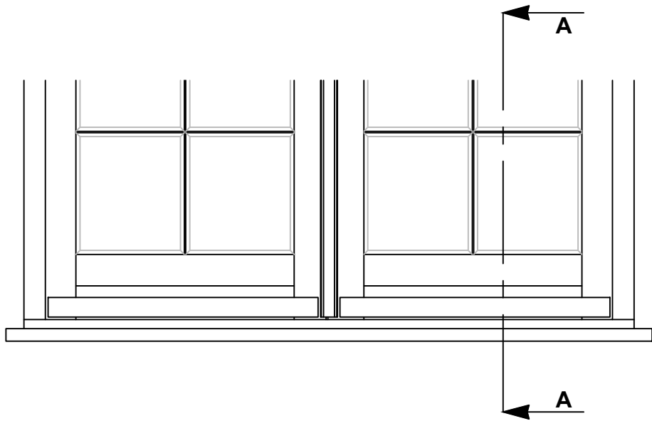
35mm CILL ELEVATION WITH 50mm HORNS L+R
