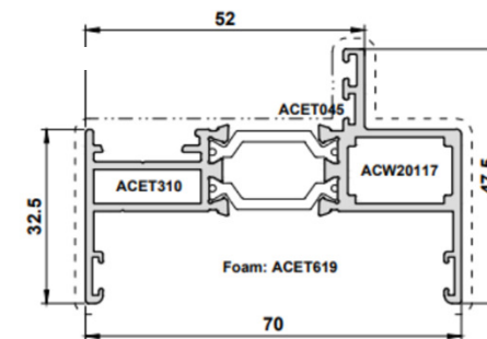
W20112 70mm Long Leg Outer Frame
