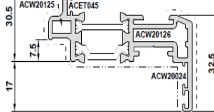
W20125 Open In Door Sash
