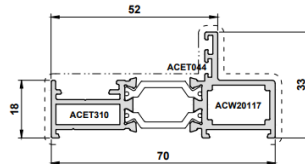
W20112 70mm Long Leg Outer Frame
