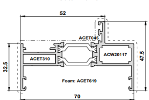
W20112 70mm Long Leg Outer Frame
