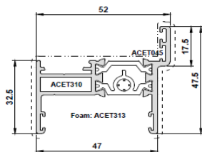
W20111 47mm Long Leg Outer Frame
