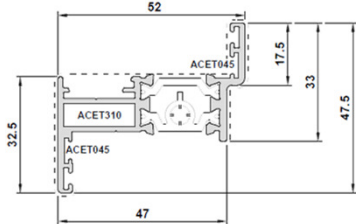
W20016 Odd Leg Outer Frame
