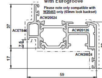
W20129 Open In Door Sash with Eurogroove
