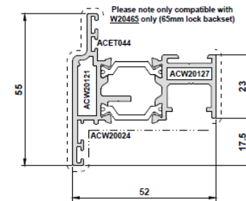
W20129 Open In Door Sash with Eurogroove
