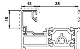
W20171N Internal Square Bead
