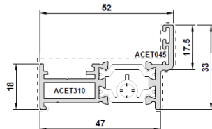
W20111 47mm Long Leg Outer Frame
