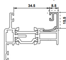
W20171N Internal Square Bead
