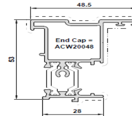
W20148 Open In Meeting Stile
