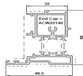
ETC371 28mm Square Bead
