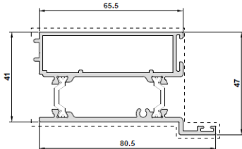
W20038 Door Lock Housing
