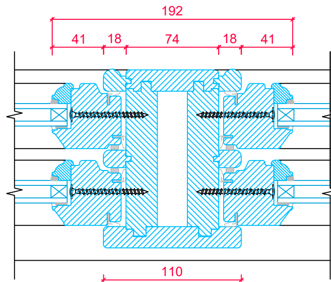
CENTRAL MULLION FOR DOUBLE FIXED SASH
