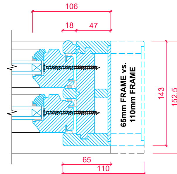
RH JAMB SECTION FOR FIXED SASH (LH IS DIRECT MIRROR)
