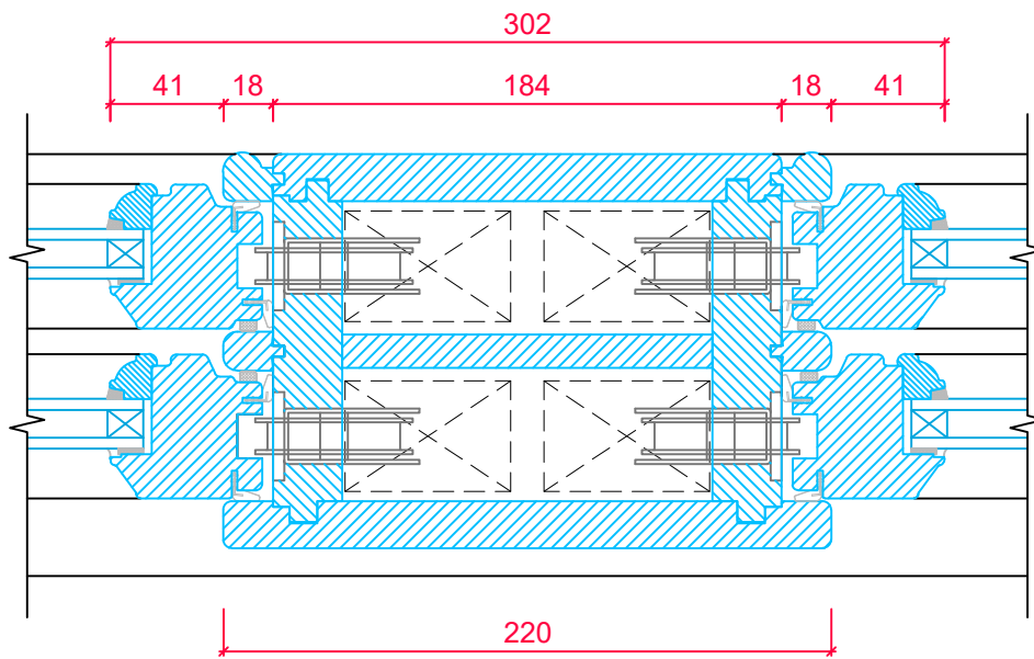
CENTRAL MULLION FOR DOUBLE OPENING SASH (both sashes open independently)
