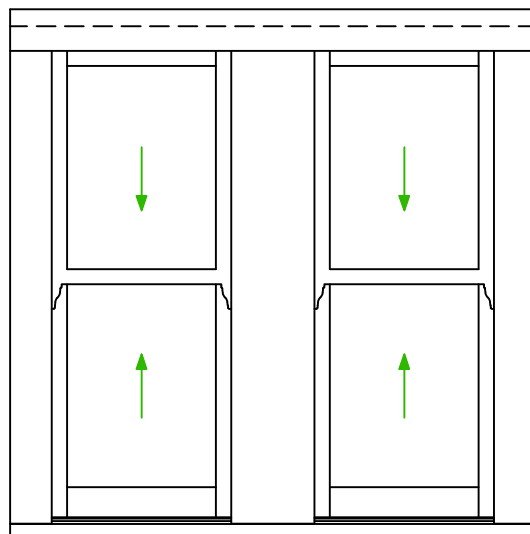
TYPICAL DOUBLE OPENING SASH LAYOUT
