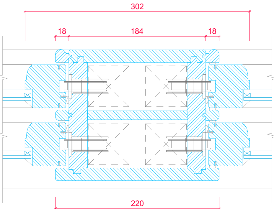
CENTRAL MULLION FOR DOUBLE OPENING SASH (both sashes open independently)
