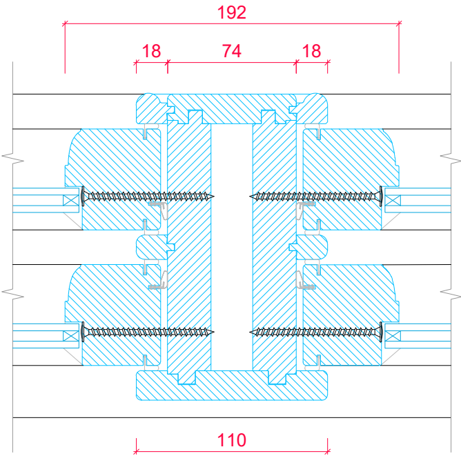
CENTRAL MULLION FOR DOUBLE OPENING SASH (both sashes open independently)
