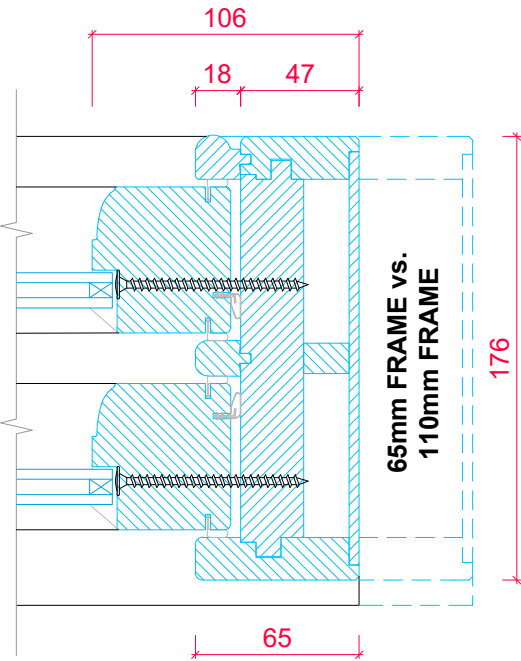
CENTRAL MULLION FOR DOUBLE OPENING FIXED COMBO SASH
