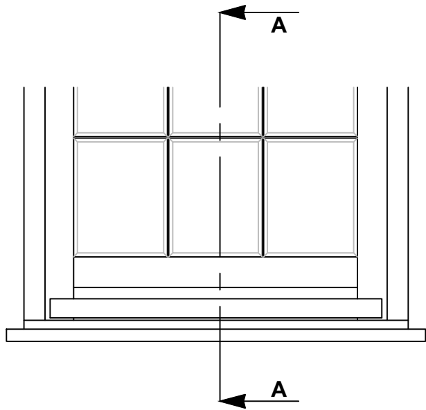
35mm CILL ELEVATION WITH 50mm HORNS L+R
