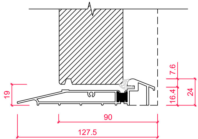
ALUMINIUM THRESHOLD SECTION 'B-B'
