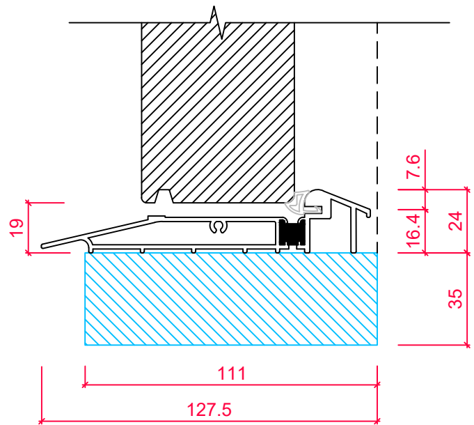
FLUSH CILL SECTION 'A-A'
