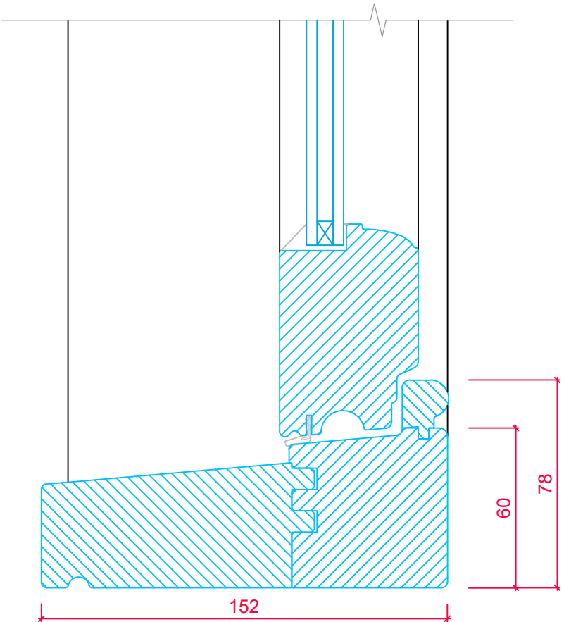
STANDARD CILL OPTION SECTION 'A-A'
