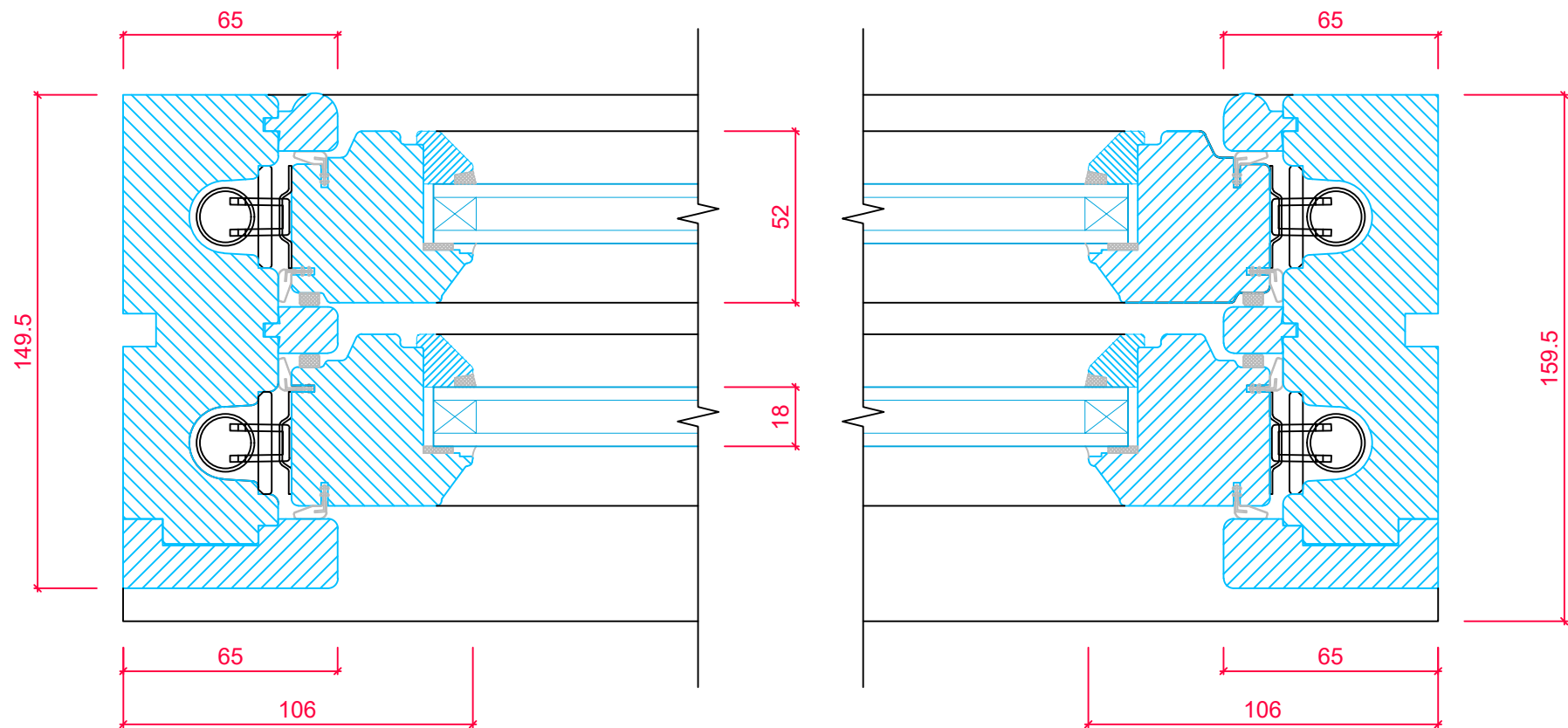
SASH CROSS SECTION 'A-A'
