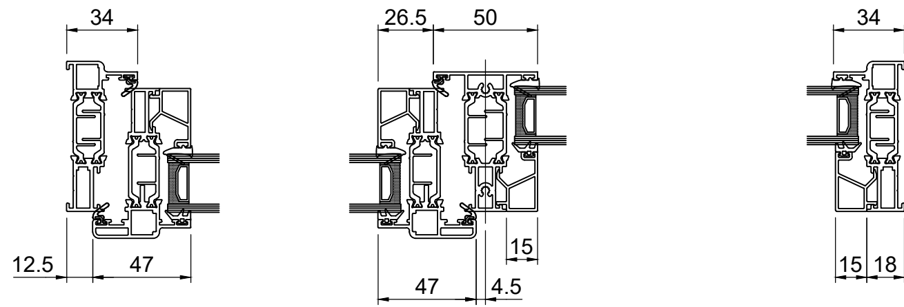
SECTION B-B
