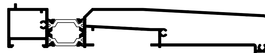
165mm DROP NOSE SILL WP 0024 - 165
