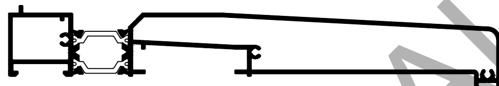
195mm DROP NOSE SILL WP 0024 - 195
