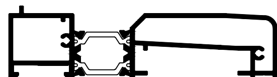
105mm SILL WP0024 - 105
