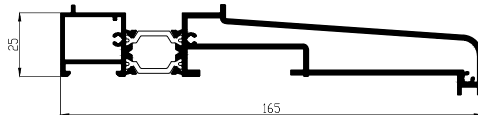
165mm DROP NOSE SILL - CONCEALED DRAINAGE AL54758
