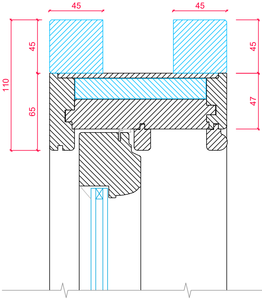
SASH CROSS SECTION 'A-A'
