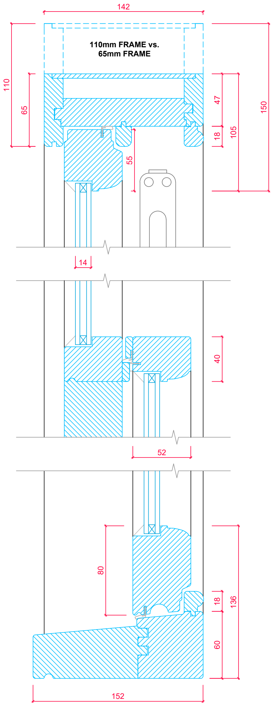
SASH CROSS SECTION 'A-A'
