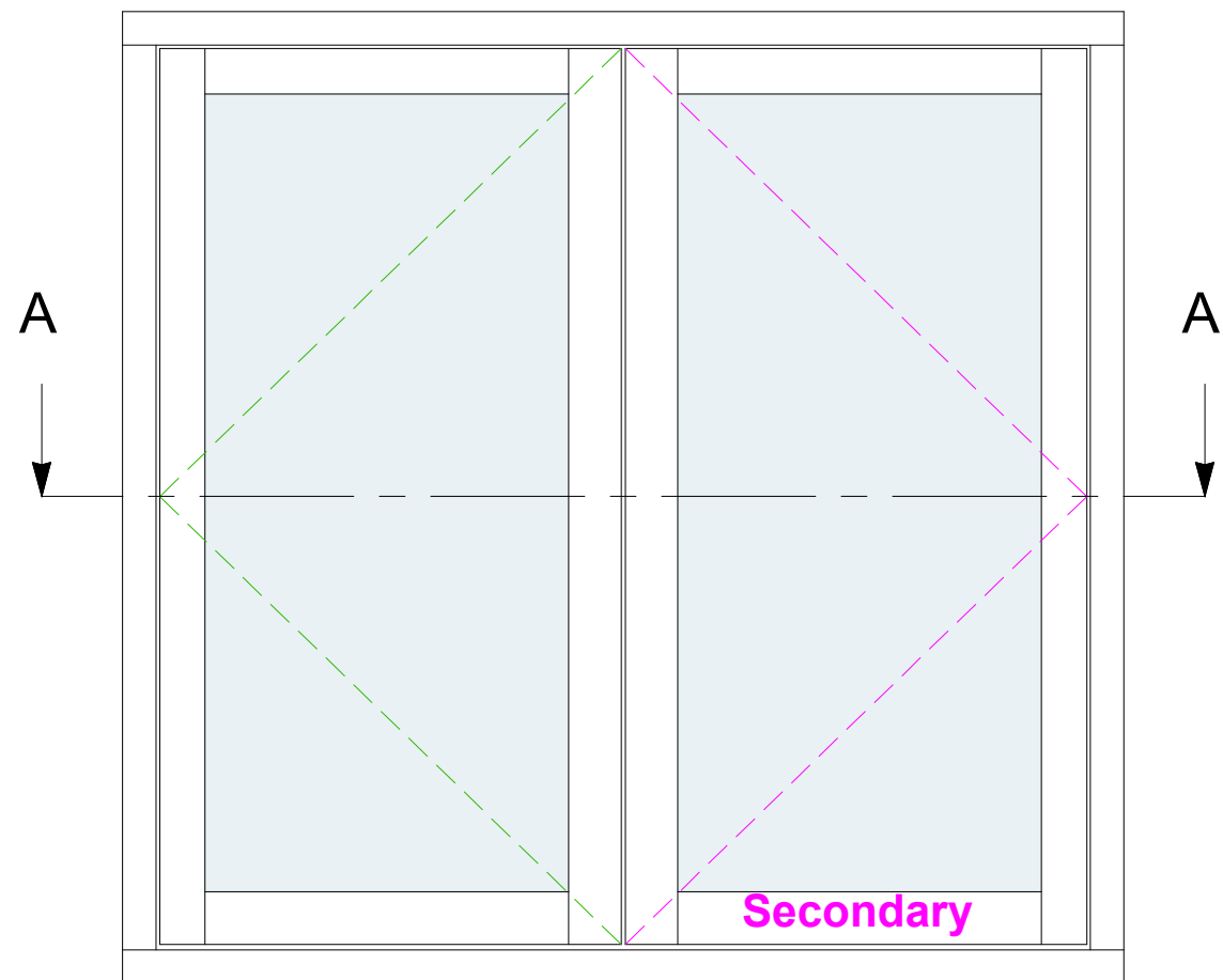
TYPICAL CASEMENT LAYOUT (SCALE 1:10)
