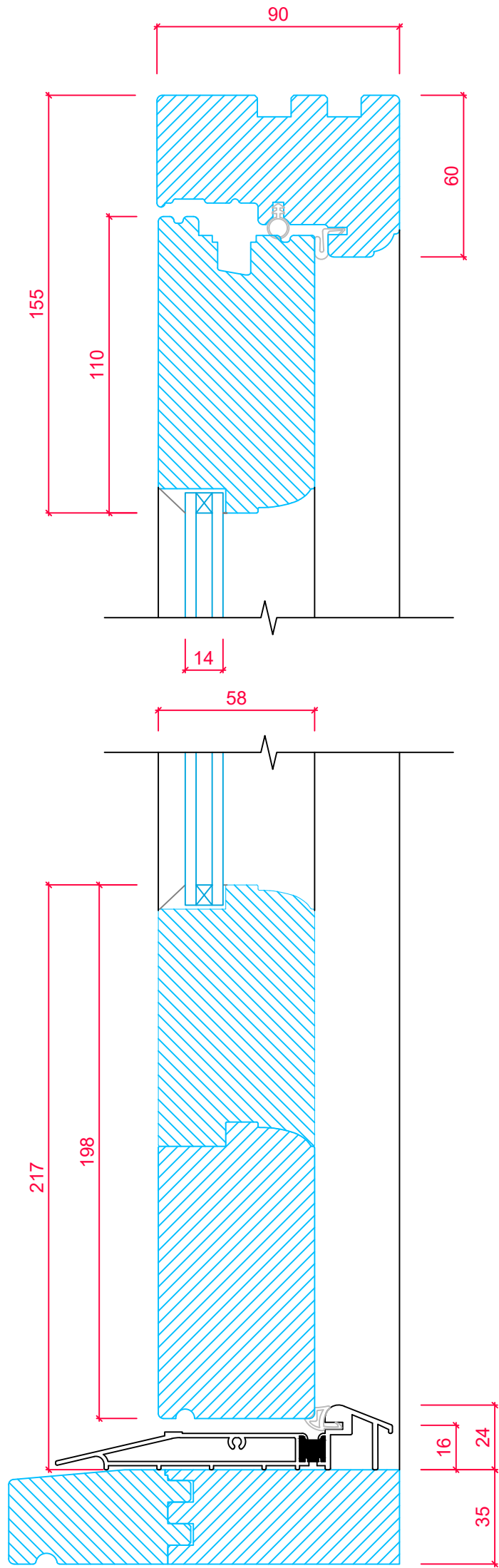
FRAME CROSS SECTION 'A-A'
