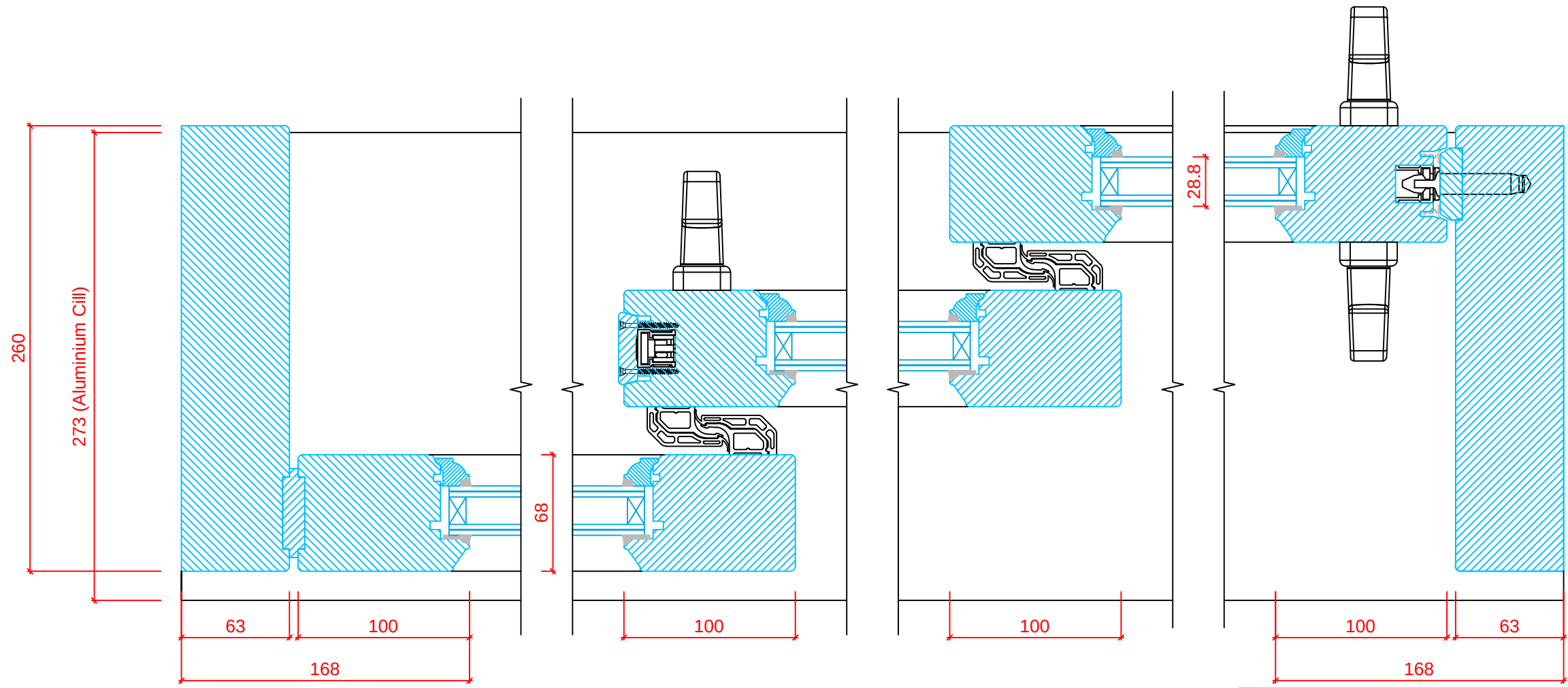
FRAME CROSS SECTION 'A-A'
