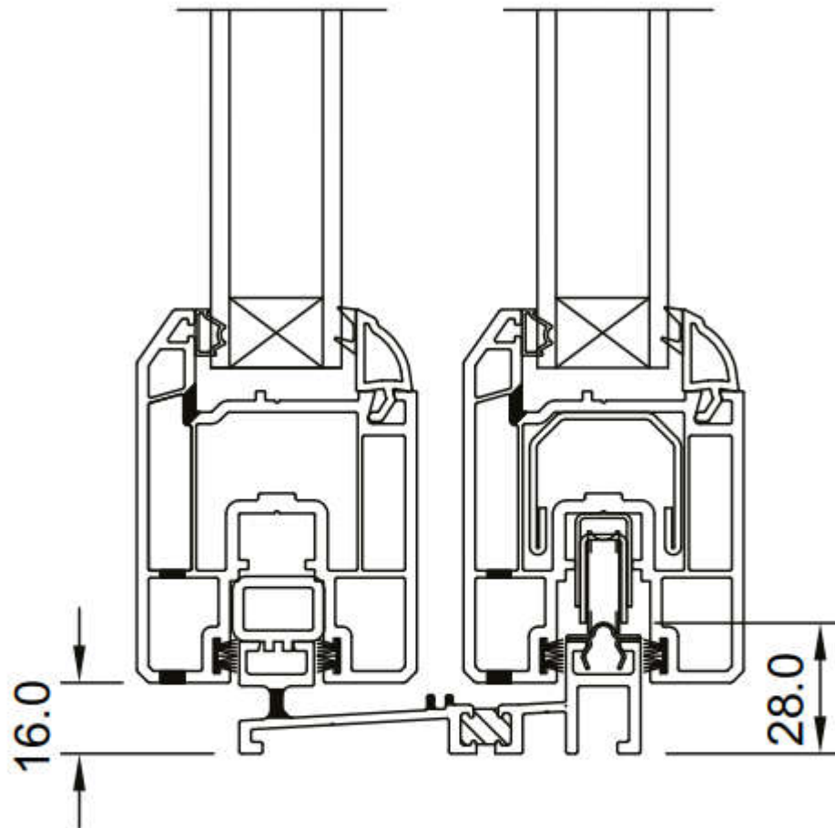
1334 - Low Threshold Thermally Broken Option
