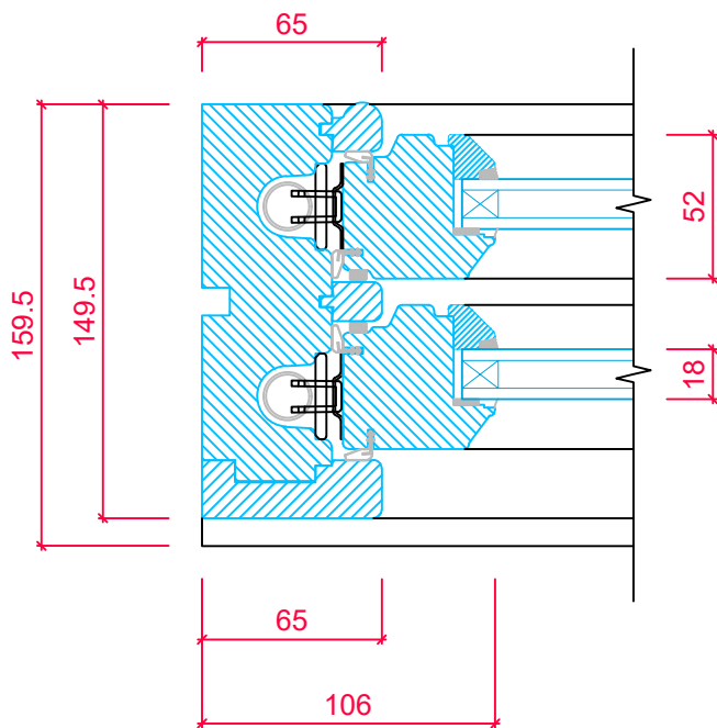
LH JAMB SECTION FOR OPENING SASH (RH IS DIRECT MIRROR)
