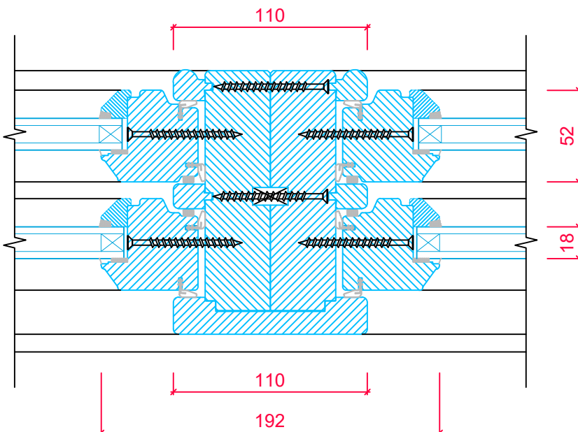
CENTRAL MULLION FOR DOUBLE FIXED SASH
