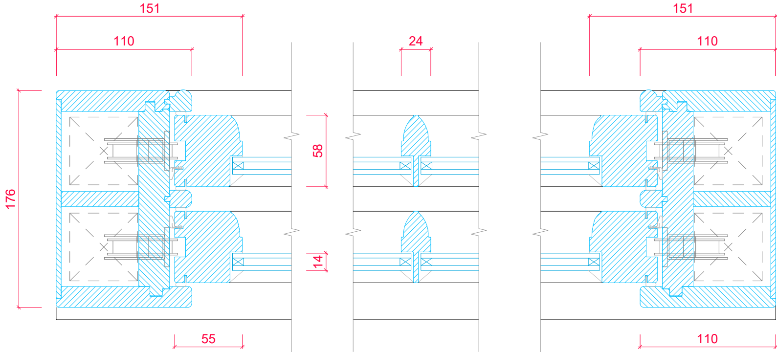
SASH CROSS SECTION 'A-A'
