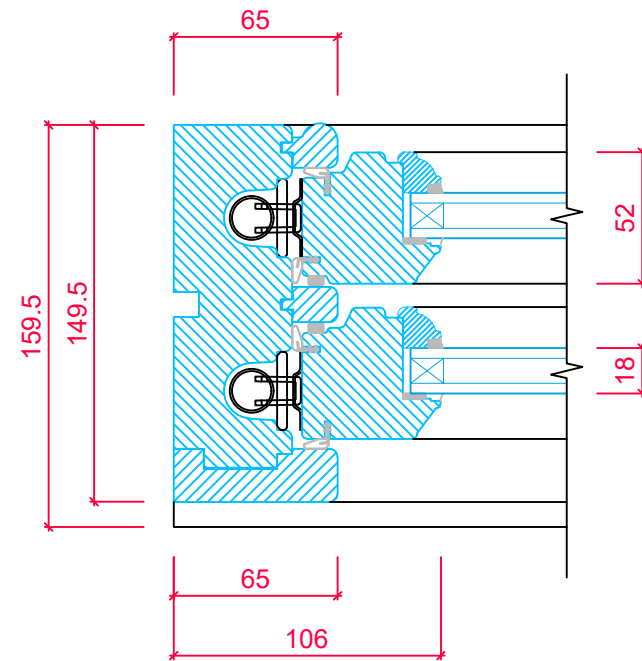
LH JAMB SECTION FOR OPENING SASH (RH IS DIRECT MIRROR)
