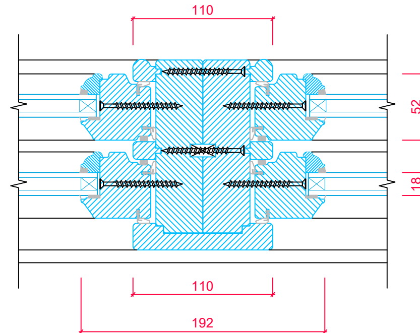
CENTRAL MULLION FOR DOUBLE FIXED SASH
