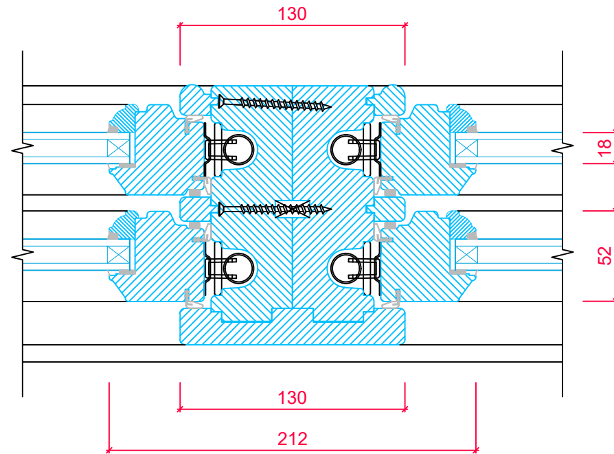
CENTRAL MULLION FOR DOUBLE OPENING SASH (both sashes open independently)
