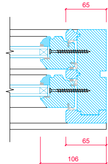
RH JAMB SECTION FOR FIXED SASH (LH IS DIRECT MIRROR)
