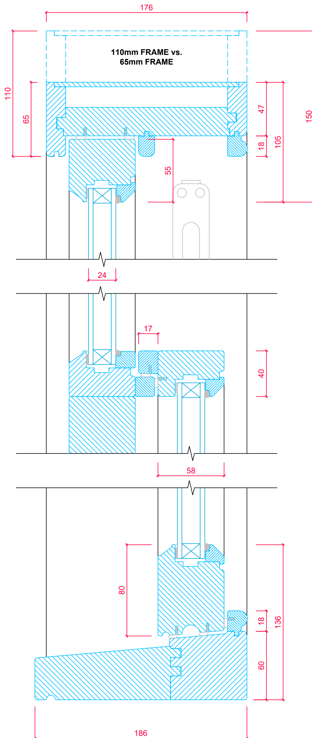
SASH CROSS SECTION 'A-A'
