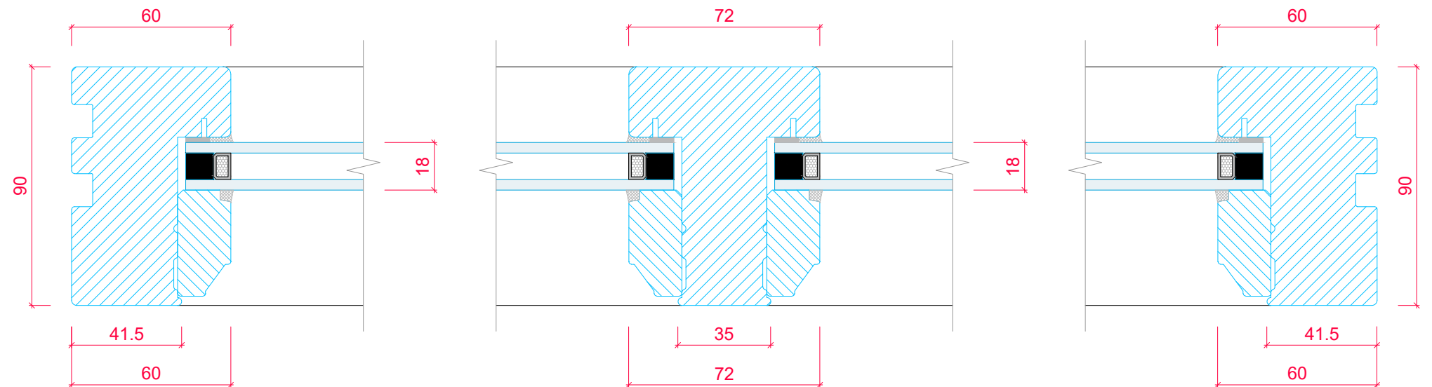
CASEMENT CROSS SECTION 'A-A' (SCALE 1:2)
