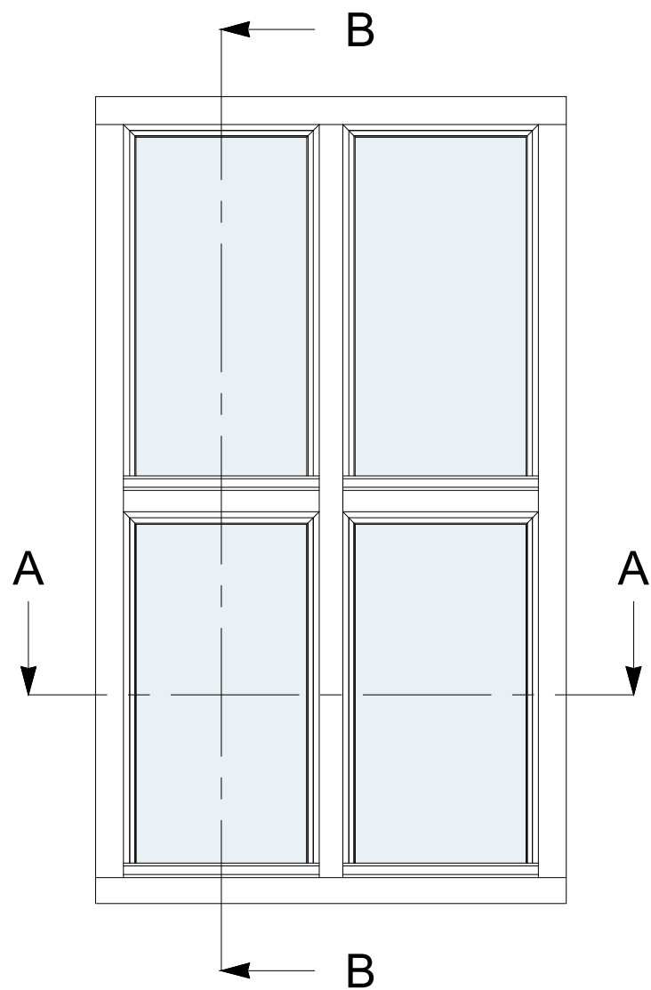
TYPICAL CASEMENT LAYOUT (SCALE 1:10)
