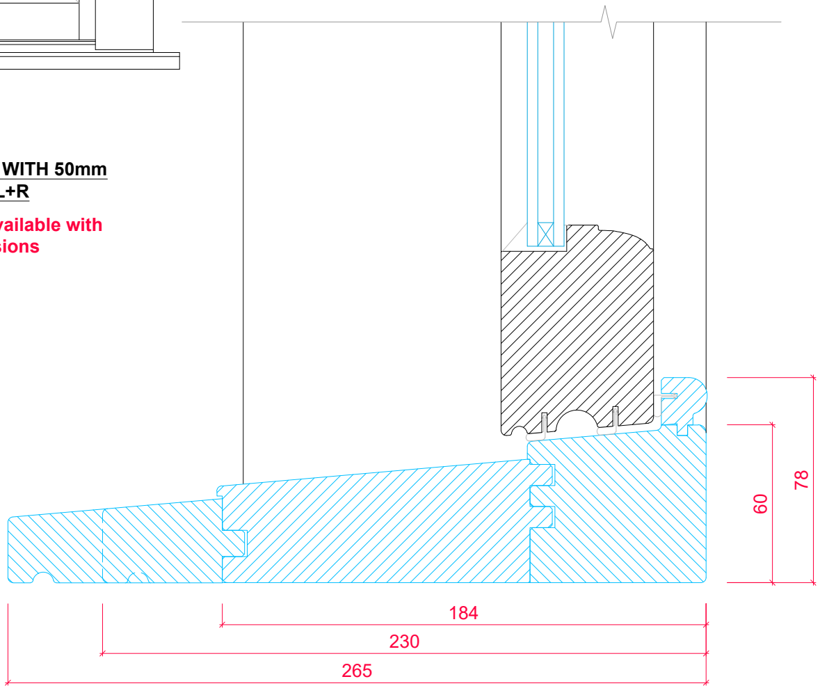
CILL EXTENSION OPTIONS SECTION 'A-A'
