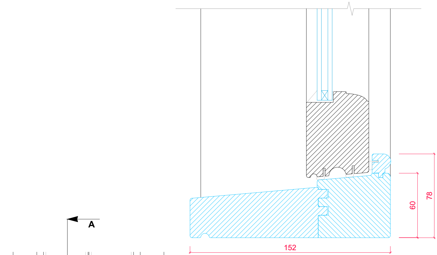
STANDARD CILL OPTION SECTION 'A-A'
