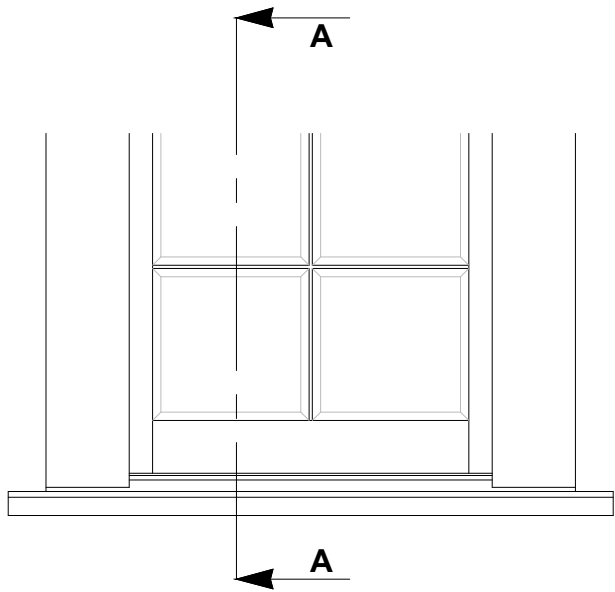
CILL ELEVATION WITH 50mm HORNS L+R
