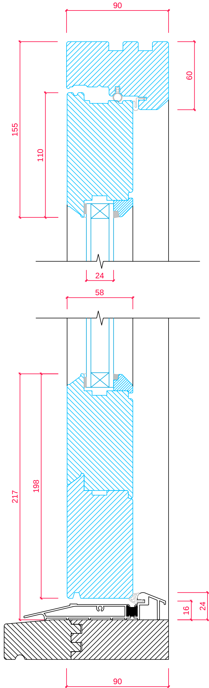
FRAME CROSS SECTION 'A-A'
