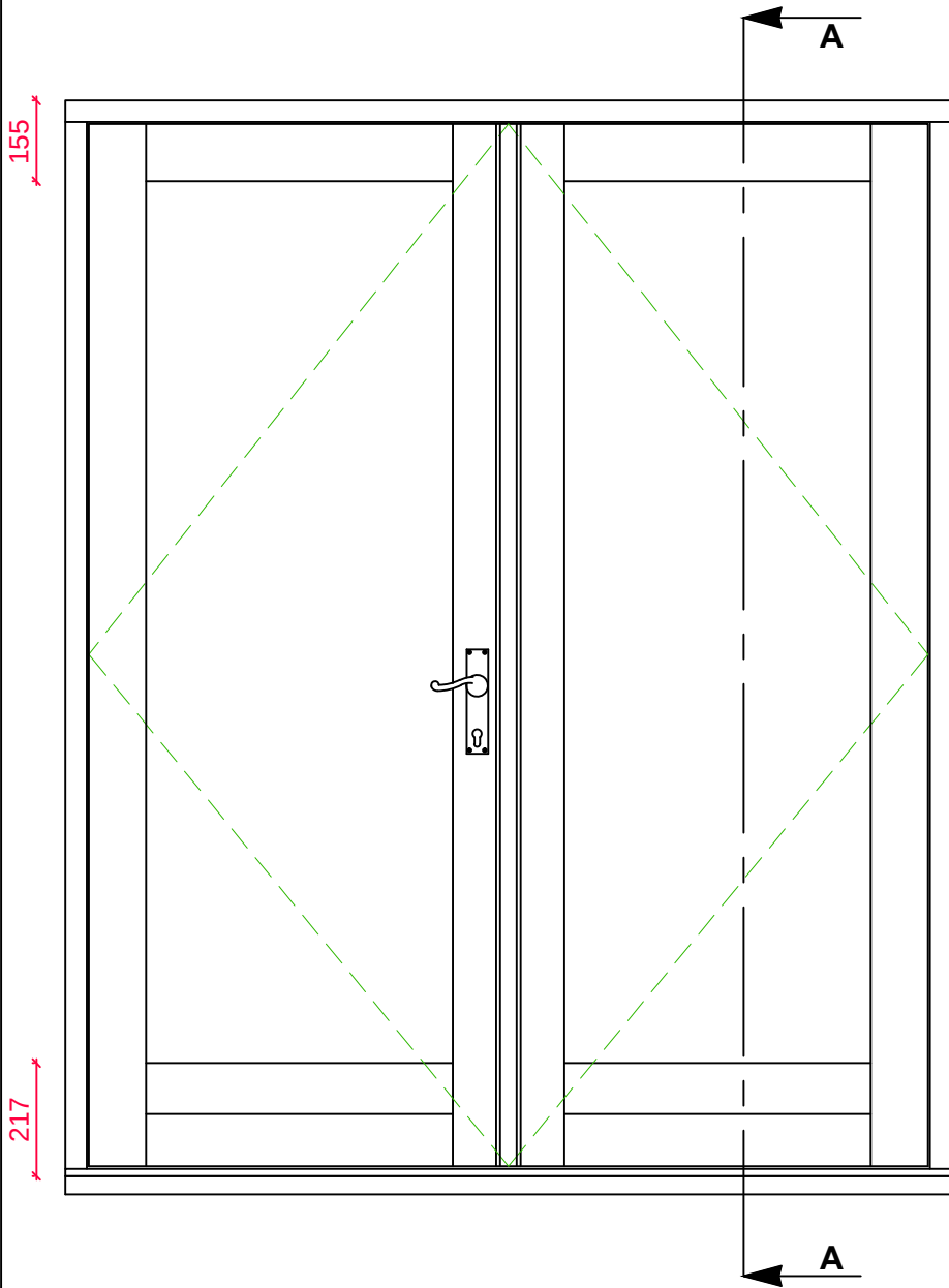
TYPICAL FRAME LAYOUT
