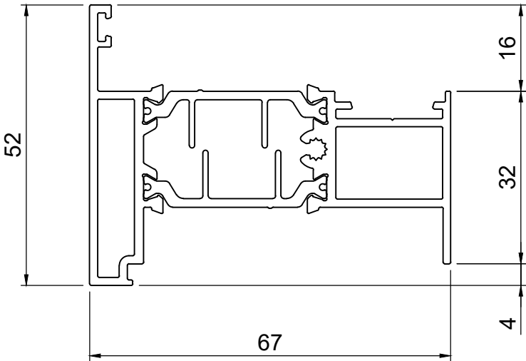
Floating Mullion
