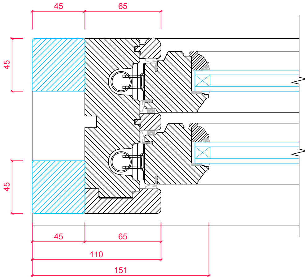
SASH CROSS SECTION 'B-B'
