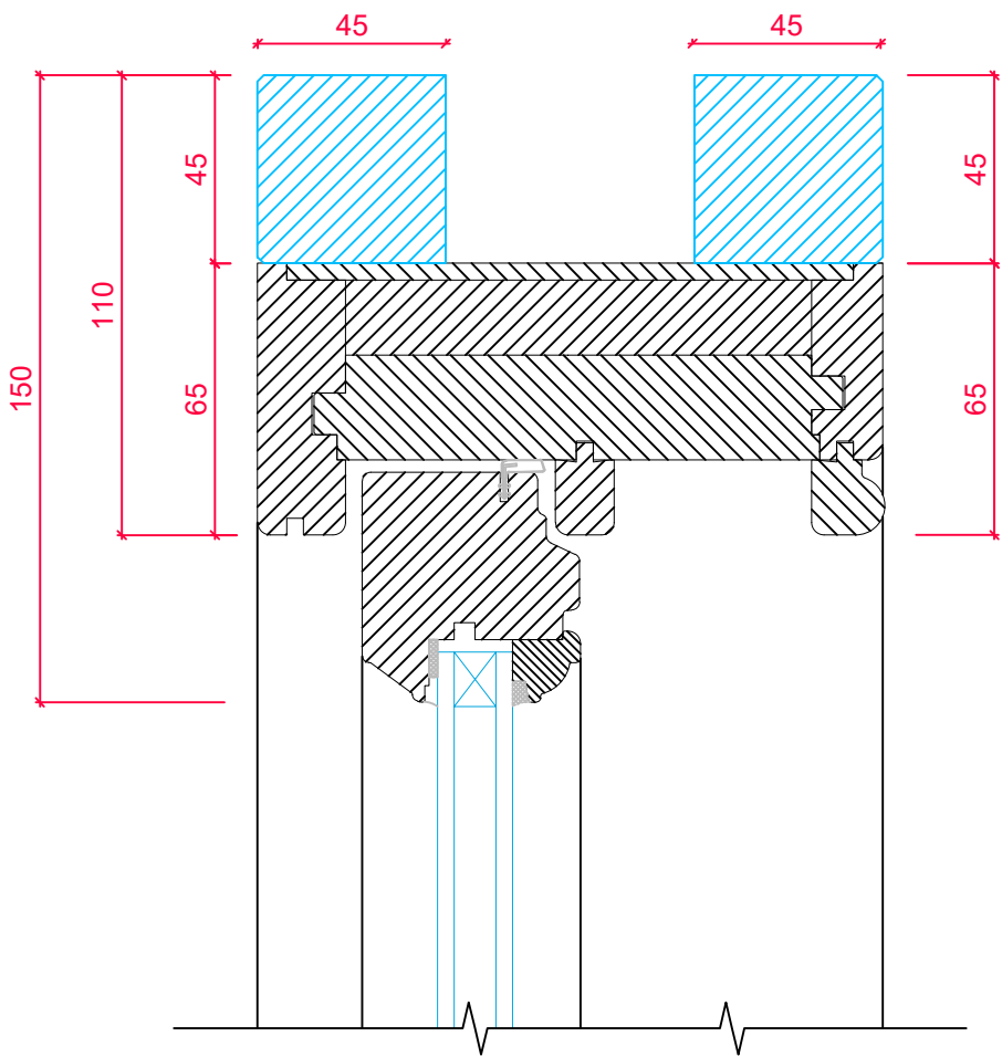
SASH CROSS SECTION 'A-A'
