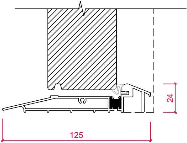
ALUMINIUM THRESHOLD SECTION 'B-B'
