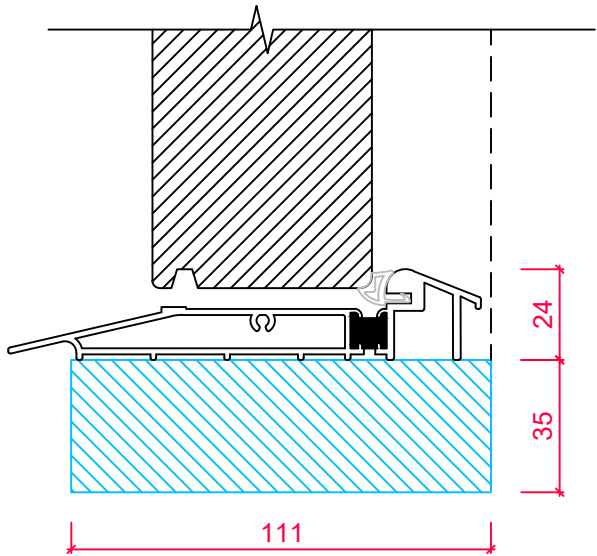
FLUSH CILL SECTION 'A-A'
