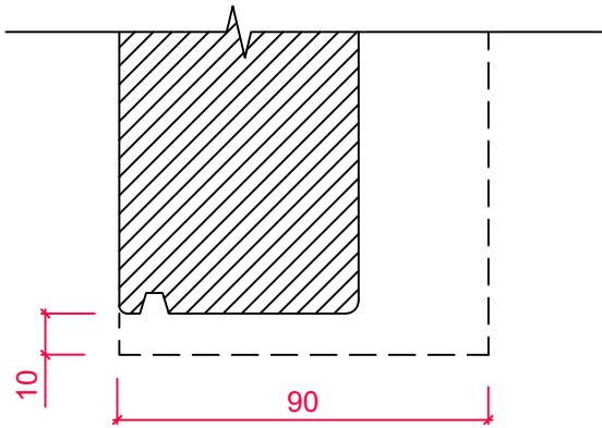
GOAL POST SECTION 'C-C'
