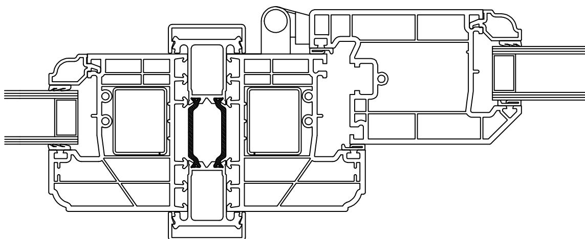
A00434 20mm Storm 2 Heavy Duty Coupler
