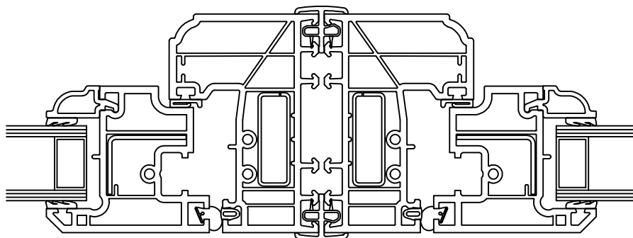
116 217 Storm 2 2mm Coupler
