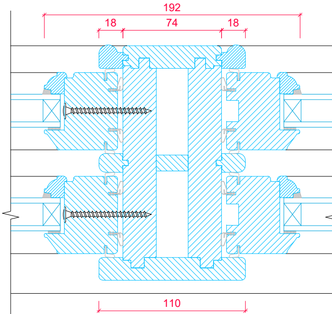
MULLION SECTION
