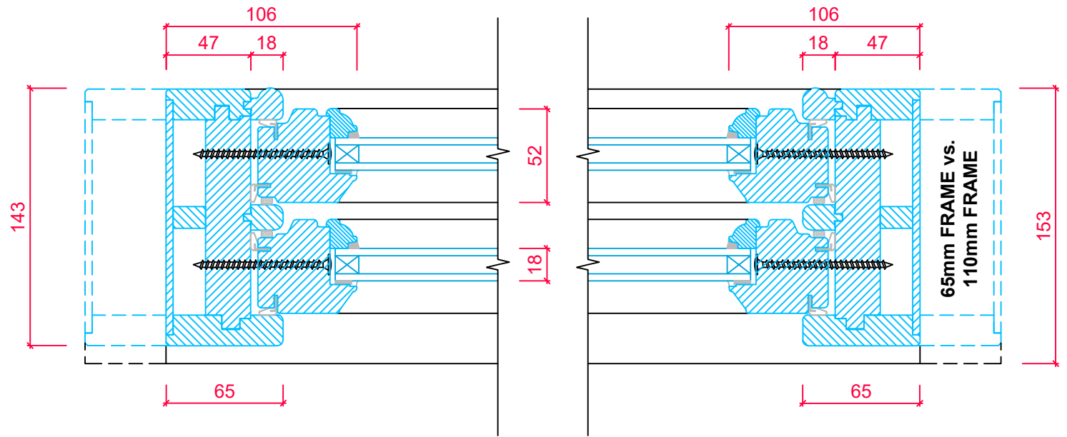
SASH CROSS SECTION 'B-B' 65mm FRAME ONLY AVAILABLE ON FIXED SASHES
