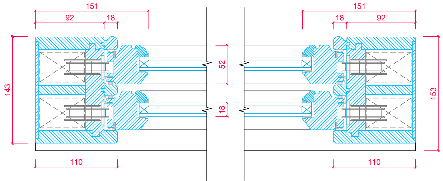
SASH CROSS SECTION 'A-A'
