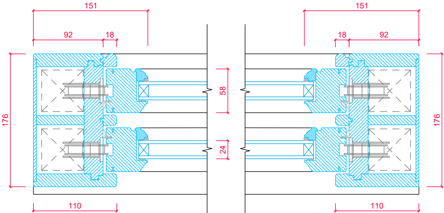
SASH CROSS SECTION 'A-A'
