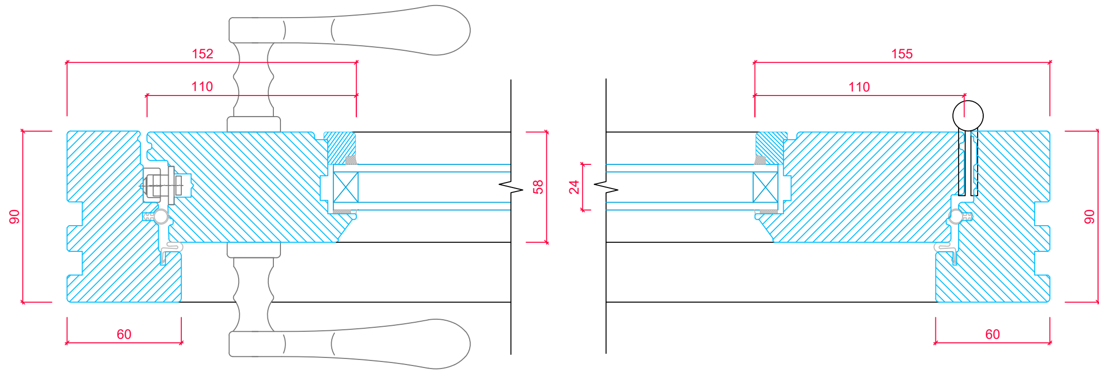
FRAME CROSS SECTION 'A-A'
