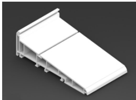
180mm integrated cill
