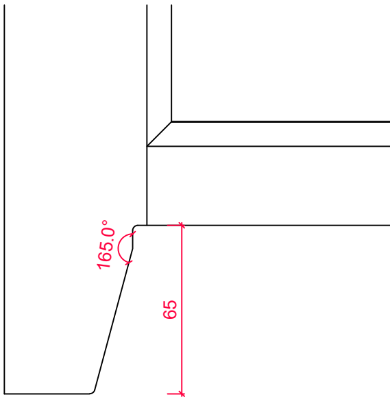
CHAMFERED
