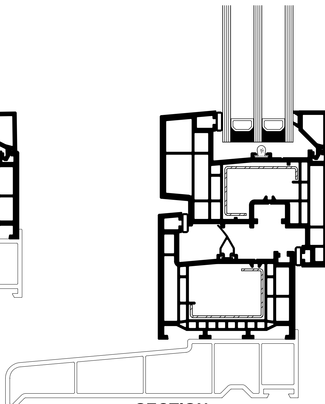
SECTION OPENING LIGHT 36mm GLAZING
