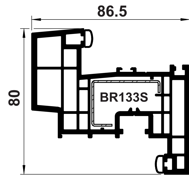
B133 TILT & TURN 'Z' SASH
