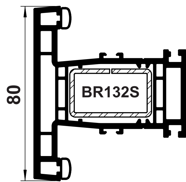
B132 'T' TRANSOM/MULLION
