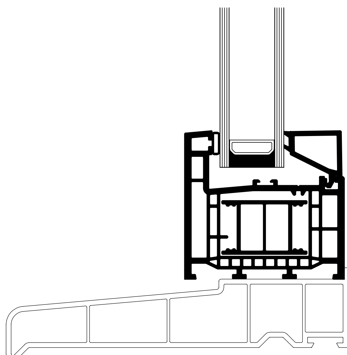
SECTION FIXED LIGHT 28mm GLAZING
