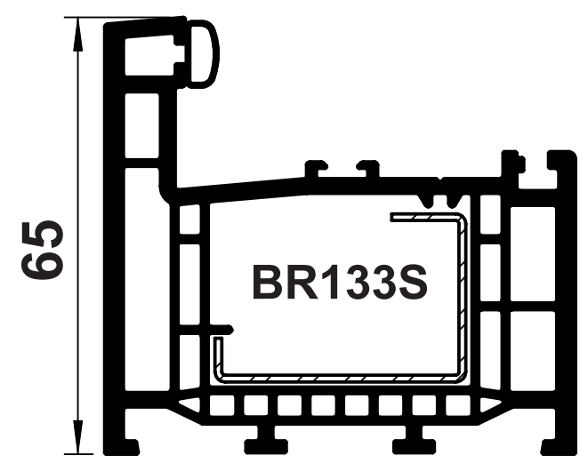
B131 OUTER FRAME
