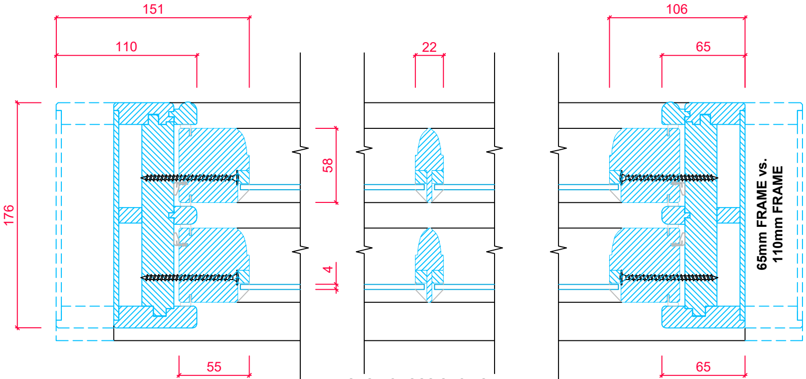
SASH CROSS SECTION 'B-B' 65mm FRAME ONLY AVAILABLE ON FIXED SASHES
