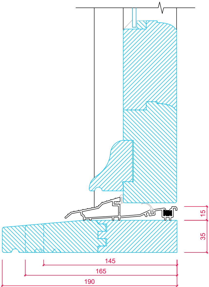
35mm CILL OPTIONS SECTION 'A-A'
