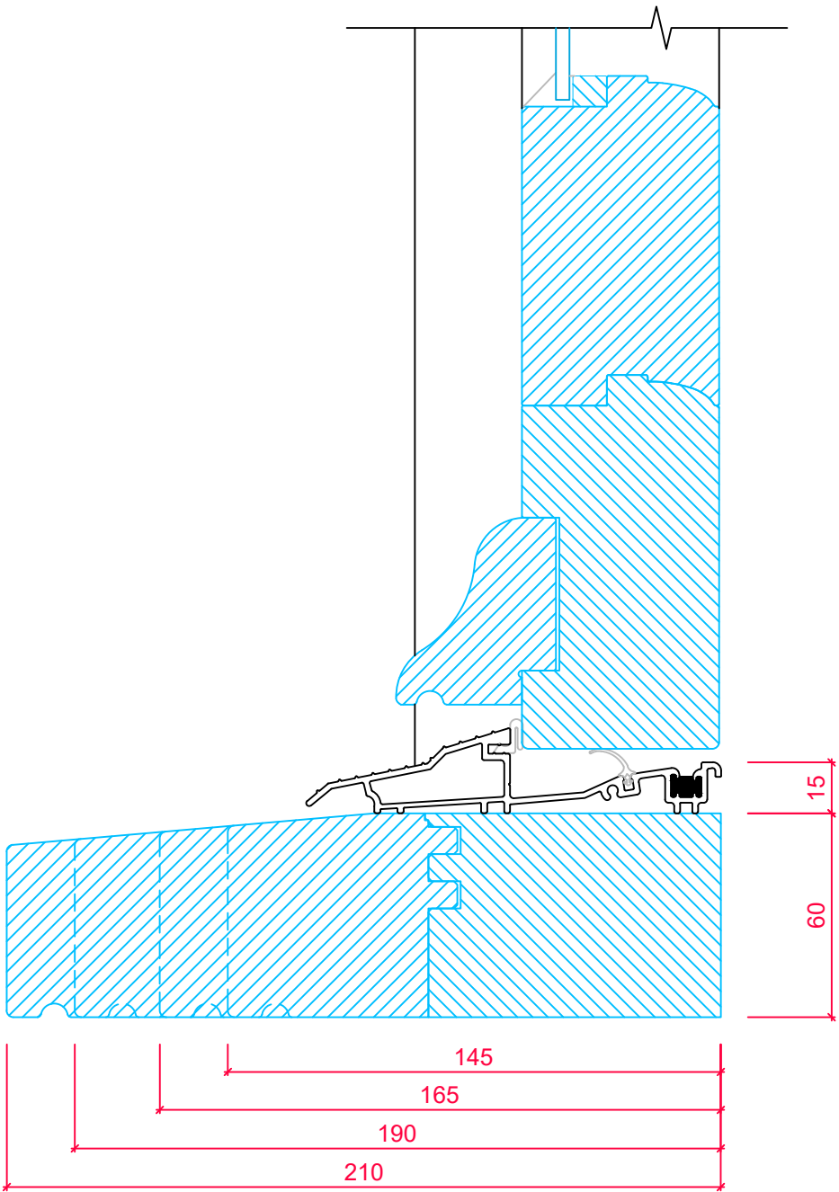
60mm CILL OPTIONS SECTION 'B-B'
