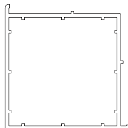
EWS120 70mm Square Corner Post
