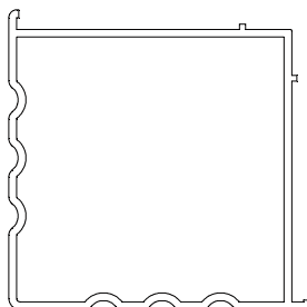
EWS130 70mm Sculptured Corner Post
