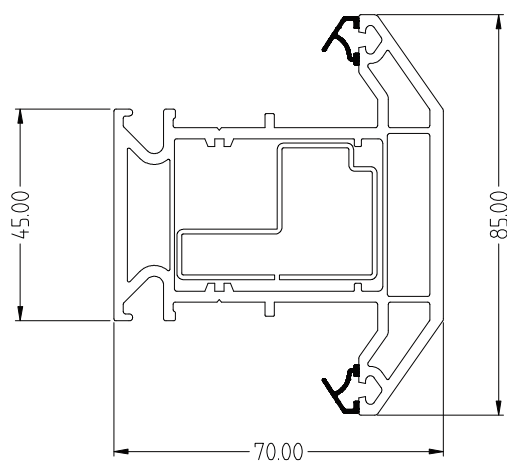
EWS7022 / 7722 Intermediate Transom 'T' & Reinforcing EWS7623S
