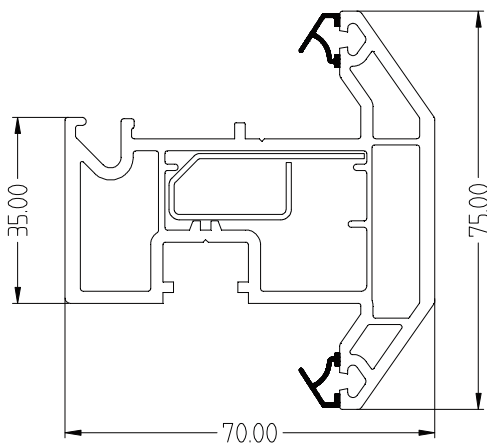
EWS7005 / 7705 Window Sash & Reinforcing EWS7604S
