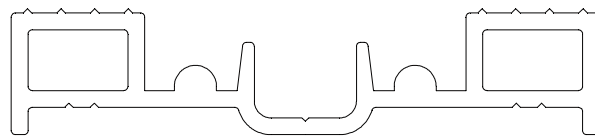
EWS7573ACH Int Room Divider Threshold
