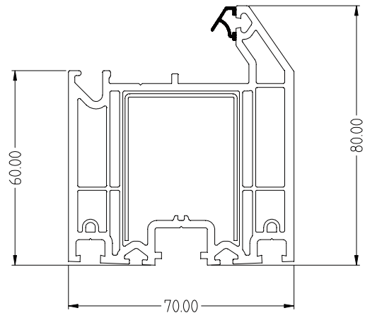
EWS7075 Door Sash & Reinforcing EWS7675S
