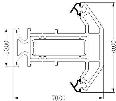
EWS7002 / 7702 Transom 'T' & Reinforcing EWS601S
