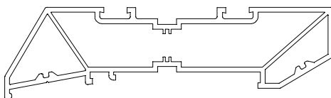
EWS135 Head Vent
