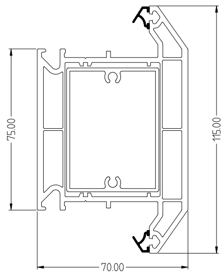
EWS7009 / 7709 Large Transom 'T' & Reinforcing EWS7509A
