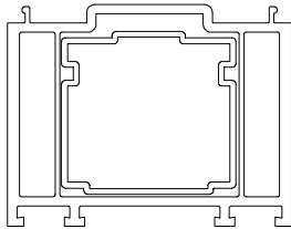
EWS126 50mm Extension & Reinforcing EWS506A
