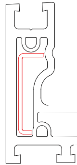
EWS7671S Outerframe Hinge Reinforcing
