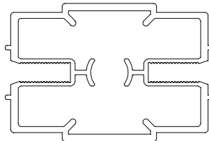
EWS528A H/Duty Butt
