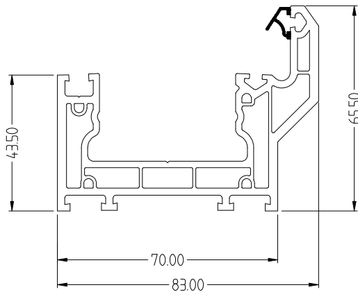
EWS7071 Outerframe
