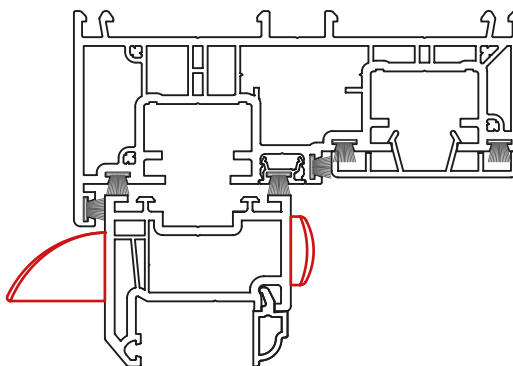
Sash vent Ultimate Rose & Heritage Rose
