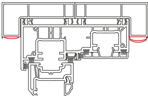
Concealed overhead vent Ultimate Rose & Heritage Rose
