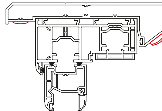
Concealed overhead vent Charisma Rose
