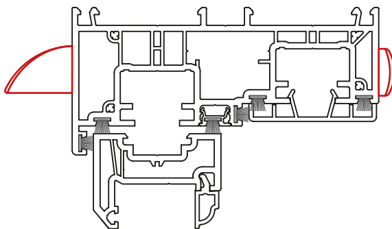
Frame vent Ultimate Rose & Heritage Rose
