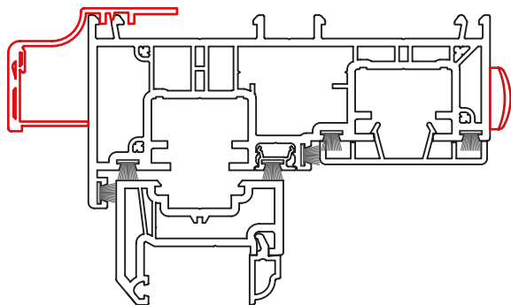
Eclipse overhead vent Ultimate Rose & Heritage Rose
