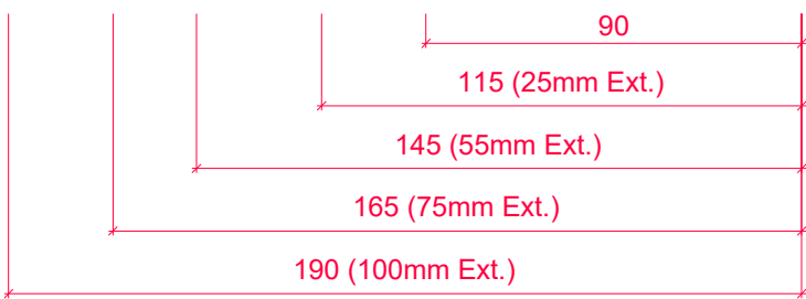
CASEMENT CROSS SECTION 'A-A' (SCALE 1:2)
